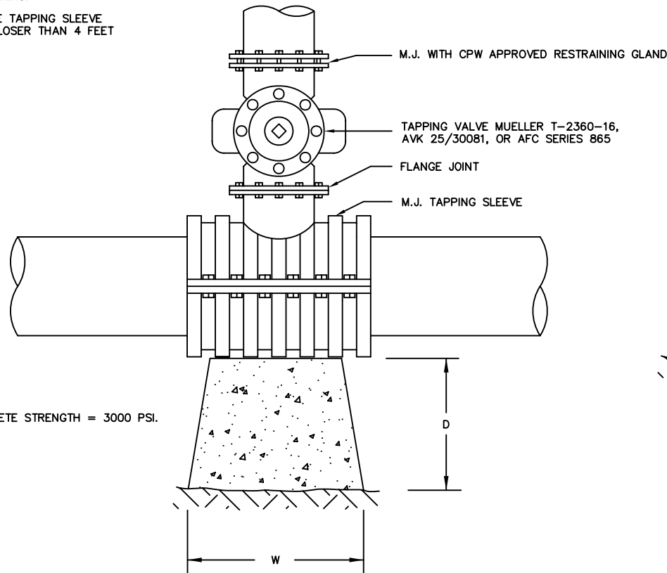
TYPICAL TAPPING SLEEVE
