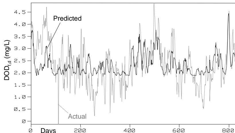
Figure 5: Actual and ANN prediction of DOD_{f,d} .
