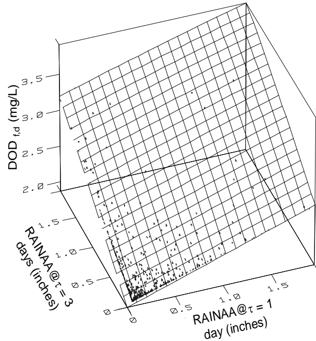
Figure 6: DOD f,d versus RAINAA @ t = 1 and 3
