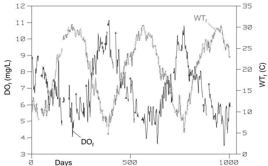
Figure 2: DO_f and WT_f for East Branch of the Cooper River (station 02172037).
