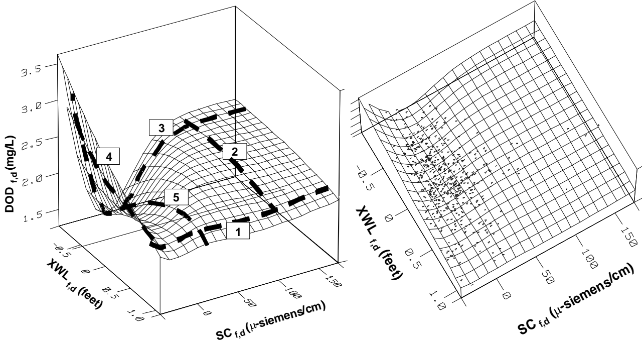
Figure 7: ANN response surface of DOD f,d versus XWL f,d and SC f,d . Different behavioral modes are marked at left. Actual values are projected onto the same surface at right, which has been tipped to show the distribution of the data.
